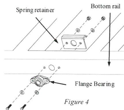
Cut-away assembly view, do not cut bottom rail!!
